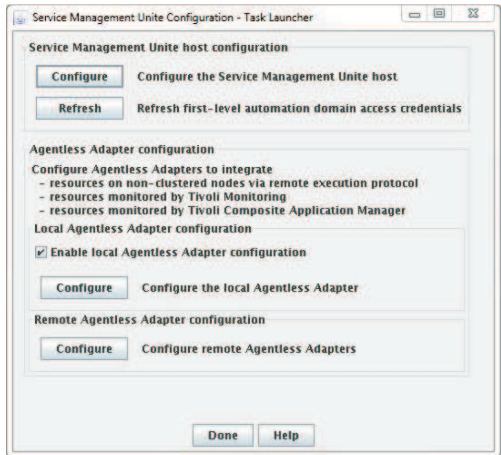
Figure 3. IBM Service Management Unite configuration - main menu
