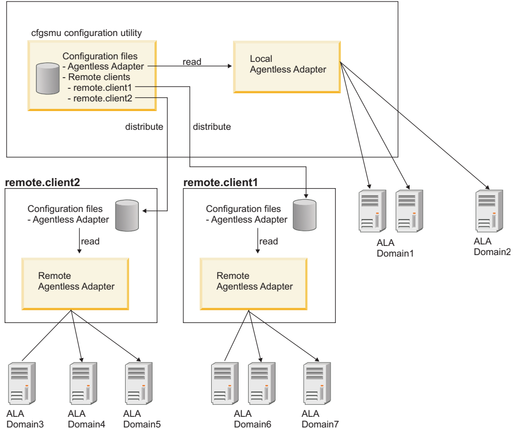
Figure 4. Maintaining configurations for multiple agentless adapters
